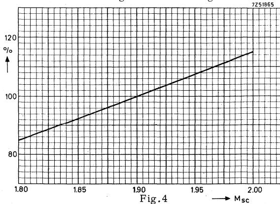
Line-width as a function of the scan-magnification factor (approximately) Line-width at M_{sc} = 1.9 is 100%, I_{screen} = \text{const.}
