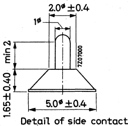
Detail of side contact
